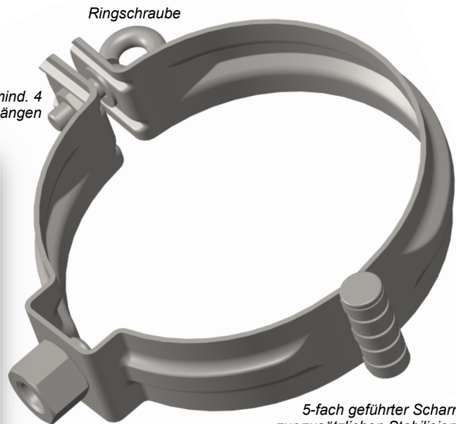
M10 Mutter
